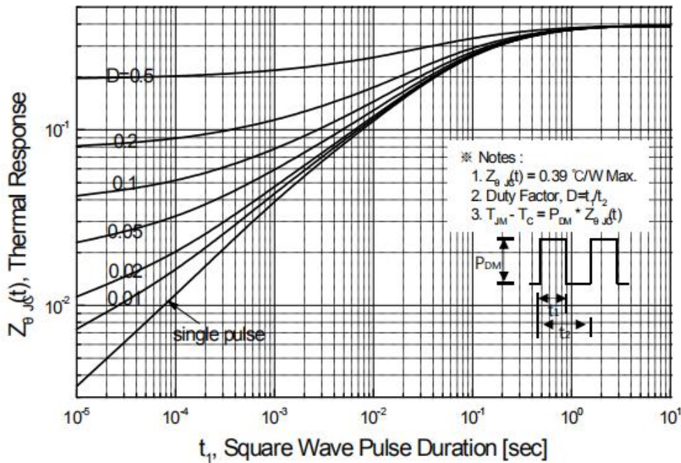
Figure 11. Transient Thermal Response Curve
